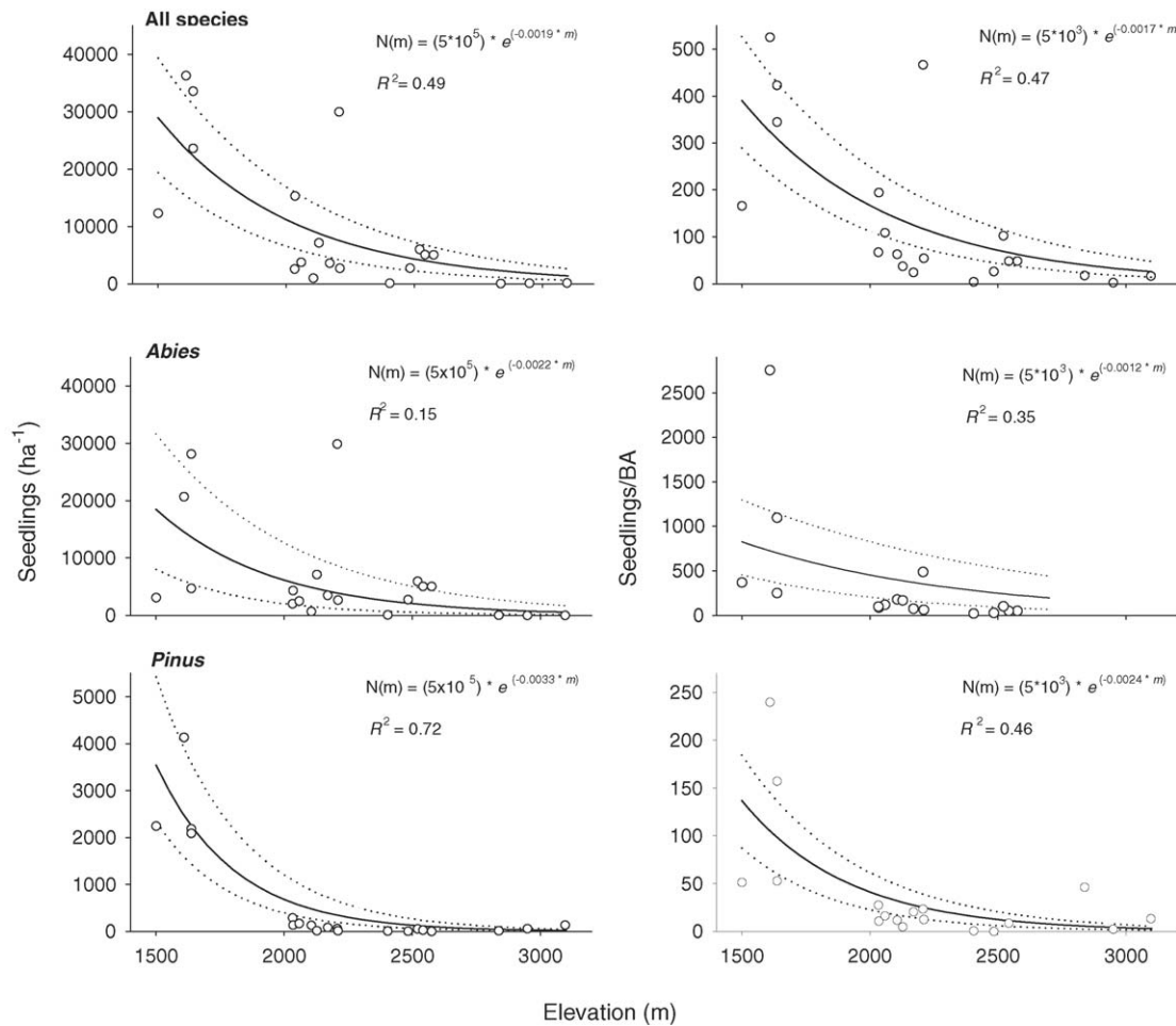
Fig. 1. Relationship between elevation and the average number of seedlings ( \text{ha}^{-1} ) from 1999 to 2003 for all species, Abies and Pinus . The relationships are also shown relative to the basal area ( \text{m}^2 \text{ha}^{-1} ) of potential parent trees (seedlings/BA). The solid line is the regression estimate, with the dashed lines showing the 95% confidence intervals calculated from 5000 bootstrapped estimates. N(m) is the number of seeds or seedlings at a given elevation and m is the elevation (meters). Note the different scales for the vertical axes.
