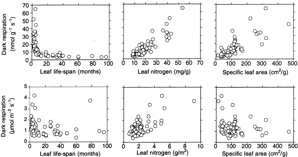
Fig. 1 Mass- and area-based dark respiration rates for 69 species from six biomes pooled, in relation to leaf life-span, mass- and area-based leaf N, and specific leaf area (SLA, cm 2 /g)
