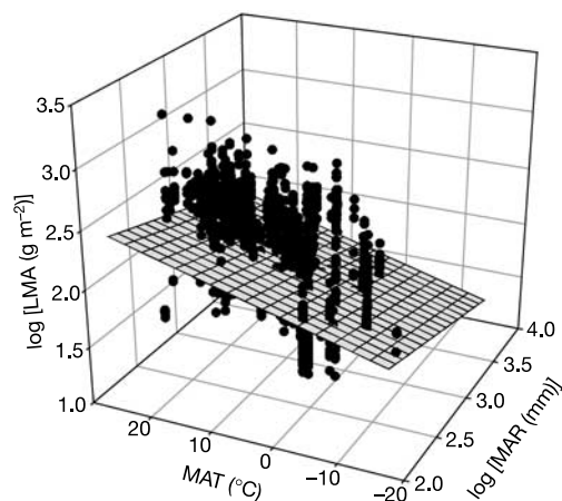
Figure 3 LMA as a function of MAT and MAR at the study sites (data for 2,370 species from 163 sites; rainfall and LMA are log 10 -scaled). The coefficients for MAT and log rainfall were highly significant in a multiple regression (both P < 0.0001 ; further details given in Supplementary Information).
