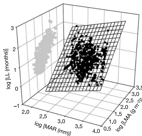
Figure 4 LL as a function of LMA and MAR (all axes are log 10 -scaled). When viewed in three dimensions, the two-dimensional LL–LMA cloud of points is spread along a sloping surface. The slope of this surface is steeper in the LMA dimension than in the rainfall dimension, reflecting the higher partial regression coefficient for LMA (1.23 versus 0.47). Both coefficients were highly significant in a multiple regression ( P < 0.0001 ; r^2 = 0.51 ; data for 678 species from 51 sites).
